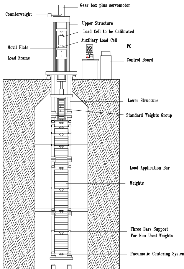
Fig. 1 CENAM's 150 kN dead weight machine.
